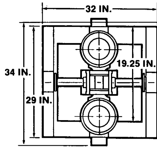
TOP VIEW (LESS TV CAMERA)
